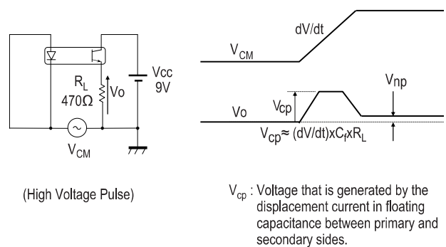
Figure 20. CMR Test Circuit
