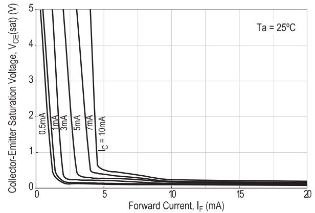
Figure 18. Collector-Emitter Saturation Voltage vs. Forward Current
