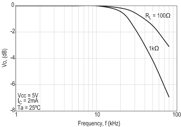
Figure 19. Frequency Response
