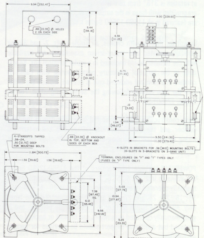
MOTOR DRIVEN
