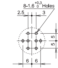
PC Board Mounting Hole Layout (Bottom View)
