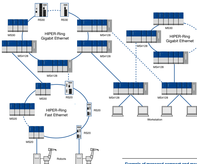
Example of managed compact and modular switches used in a HIRSCHMANN Hiper-Ring featuring Fast and Gigabit Ethernet.
