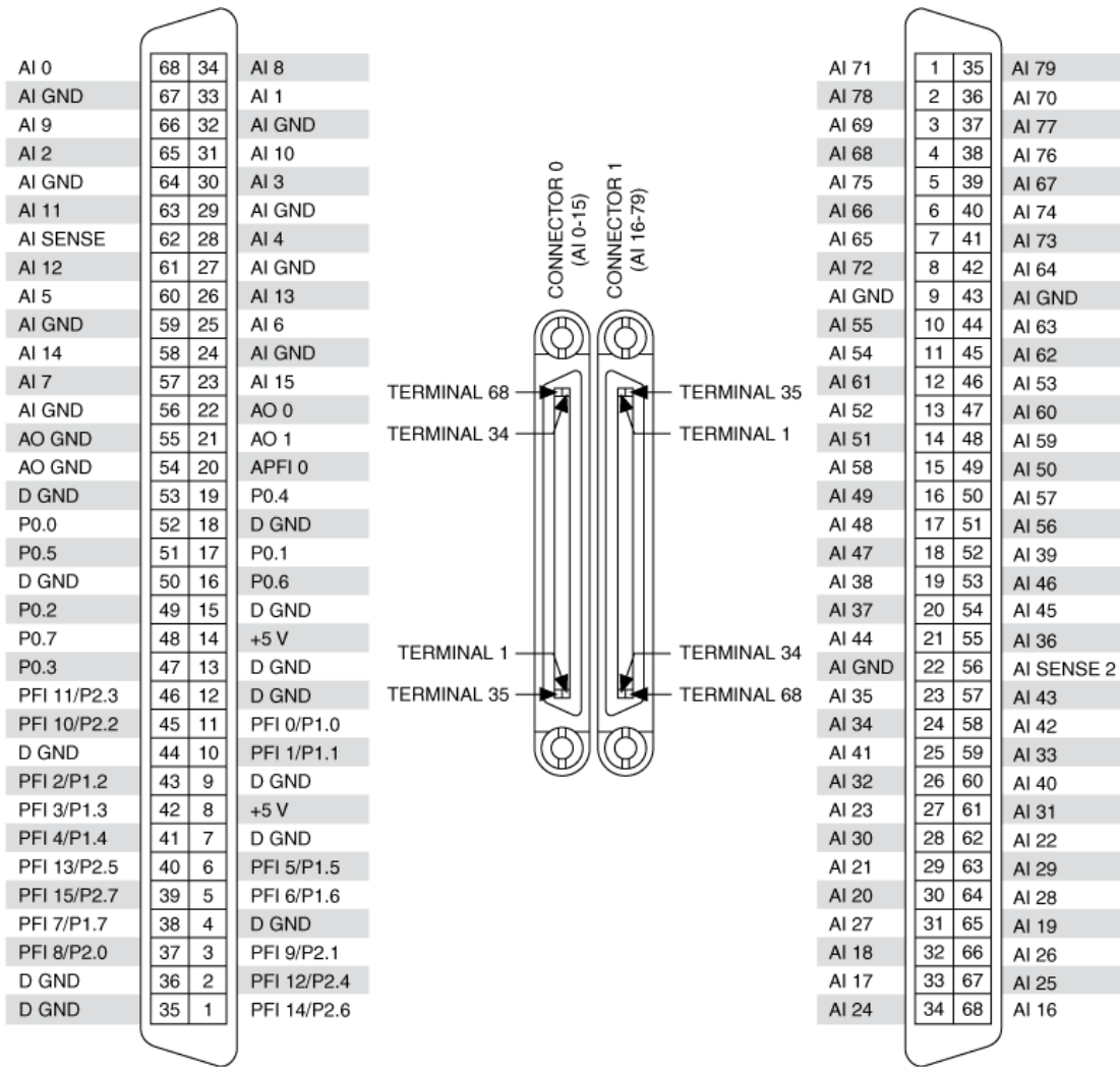
NI PCI/PXI-6255 Pinout
