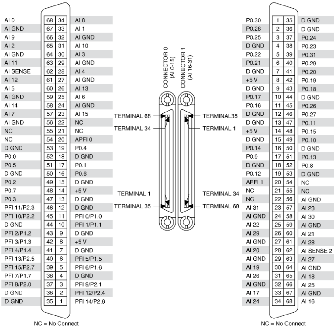
NI PCI/PXI-6254 Pinout
