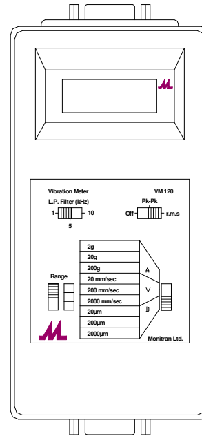
Standard Vibration Meter, Probe & Accessories
