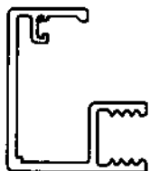
Fixed/mobile wing upright
