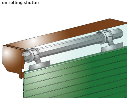
Tubular operator on rolling shutter
