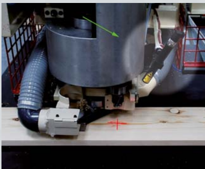
Knot drilling machine
