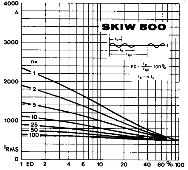
Fig. 1 b Rated rms current vs. duty cycle
