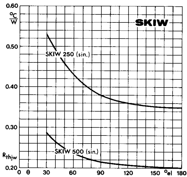
Fig. 6 Thermal resistance vs. conduction angle
