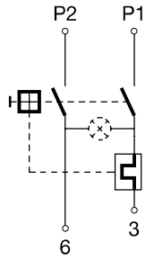
2 pole thermal overload protection, Shunt terminal Undervoltage release
