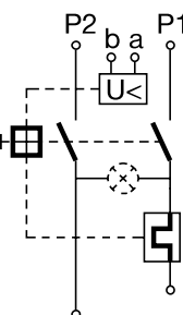
Undervoltage release with 2 additional contacts Remote trip release
