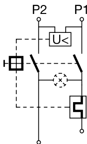
2 pole thermal overload protection, Shunt terminal Undervoltage release
