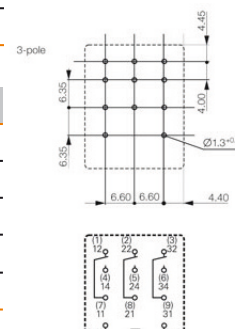
Circuit diagram View of connections Dimensions in mm
