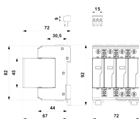
Dimension drawing
