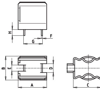
PINZE PER FUSIBILI 14x51 0900506 FUSE CLIPS FOR FUSES 14x51 0900506
