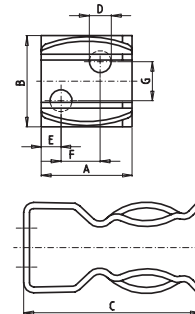
PINZE PER FUSIBILI 14x51 0900505 FUSE CLIPS FOR FUSES 14x51 0900505
