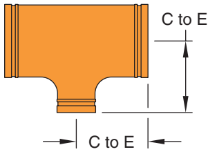
Figure 221 Reducing Tee Cast
