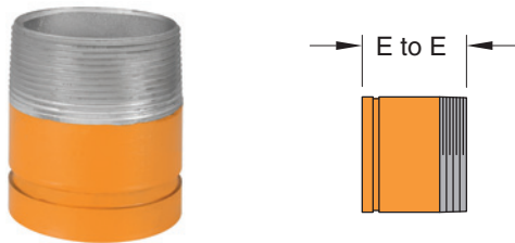
Figure 391 Fabricated Adaptor Nipple Groove x Male Thread
