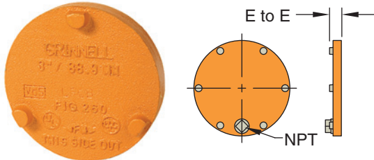
Figure 260 Cap Cast
