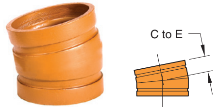
Figure 311 11 1/4° Fabricated Elbow
