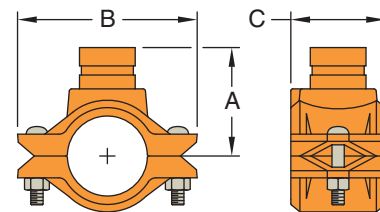
Figure 702 Outlet Coupling with Grooved Outlet
