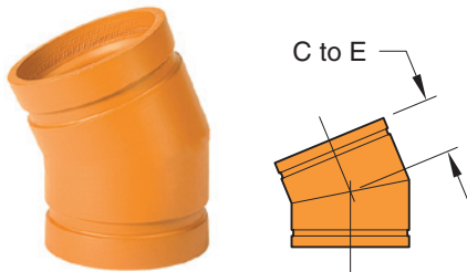
Figure 312 22 1/2° Fabricated Elbow
