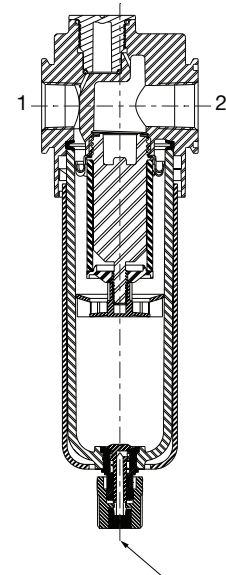
Cross Section - 651/652/653 Series Particulate Filter
