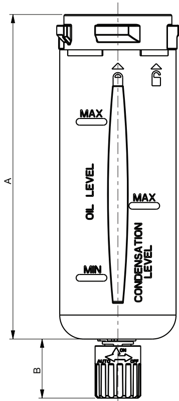
Polycarbonate Bowl/Guard with Semi-automatic/Manual Drain
