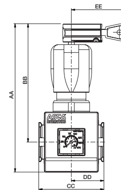
651/652/653 Series
