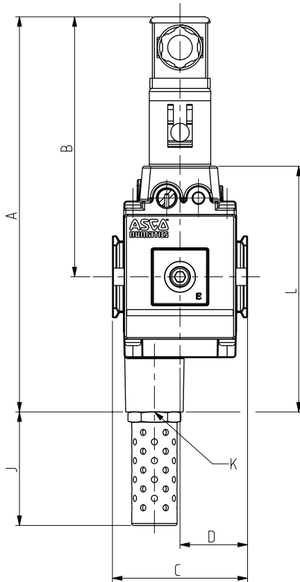
Solenoid Pilot
