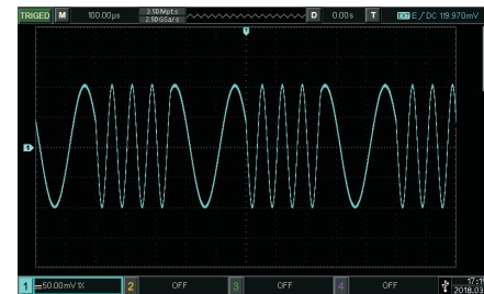
Picture 4-15 FM output waveform
