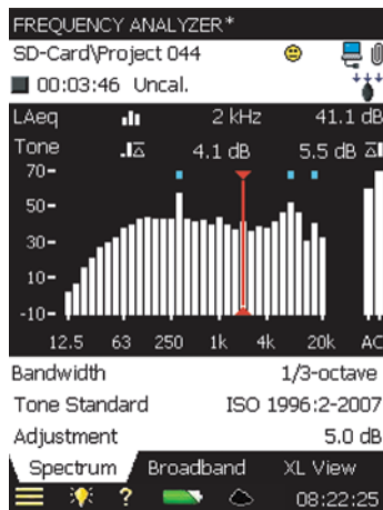
Fig. 12 Tone Assessment Option BZ-7231 showing 1/3-octave bands with audible tones higher than a set limit (tones are identified by the blue dots)
