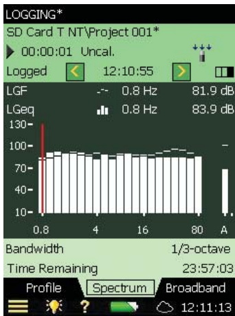
Fig. 14 Low Frequency Option showing G-weighted parameters L_{GF} and L_{Geq}
