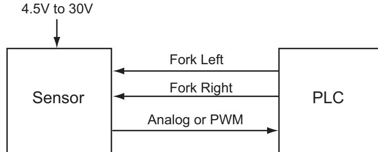
FIGURE 12. PLC interfacing
