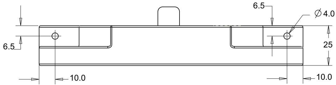
FIGURE 16. MGS1600 front view and dimensions
