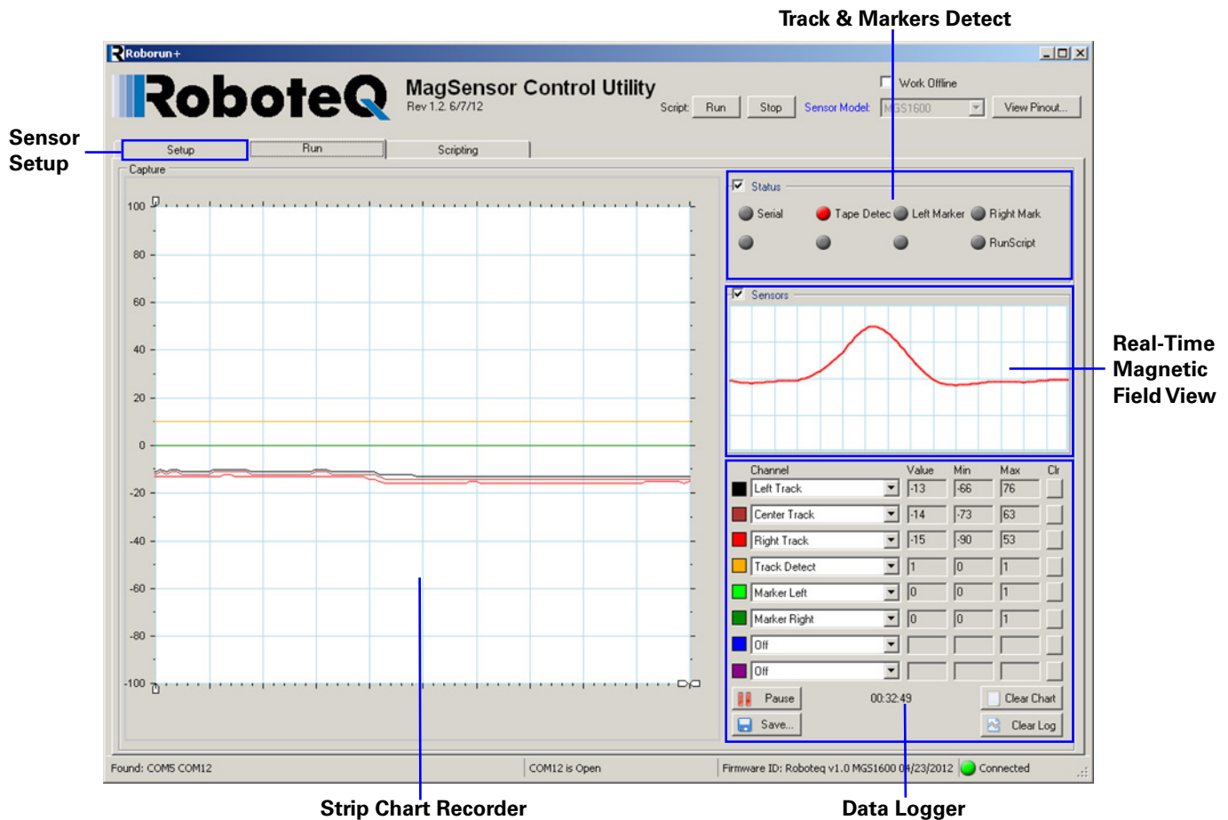
FIGURE 15. MagSensor Control Utility
