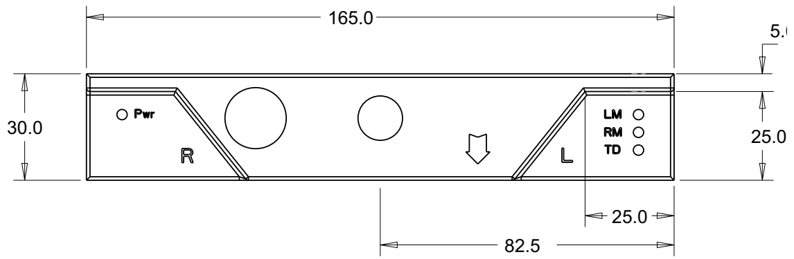
FIGURE 17. MGS1600 top view and dimensions
