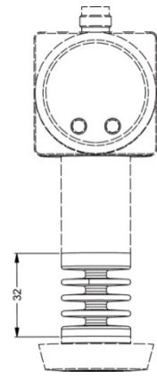
Temperaturkoppler 300 °C
